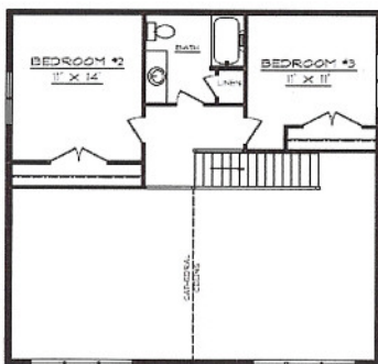
YAIL SECOND FLOOR PLAN
